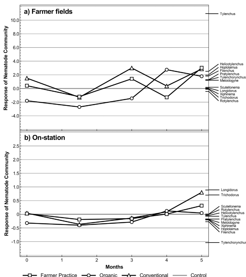
Fig. 4. Principal response curves of the plant parasitic nematode genera showing the effects of farmer practice, conventional and organic farming compared to the control from the study site in Chuka. The ordinate axis represents the first principal component of the variance due to treatment effect whereas the abscissa axis represents the sampling time (in months). The horizontal line at 0 shows the response of the plant parasitic nematodes in the control. The genera scores that were associated with the reference system (control) are shown on the right axis.
